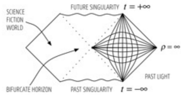
PENROSE DIAGRAM FOR BLACK HOLE
